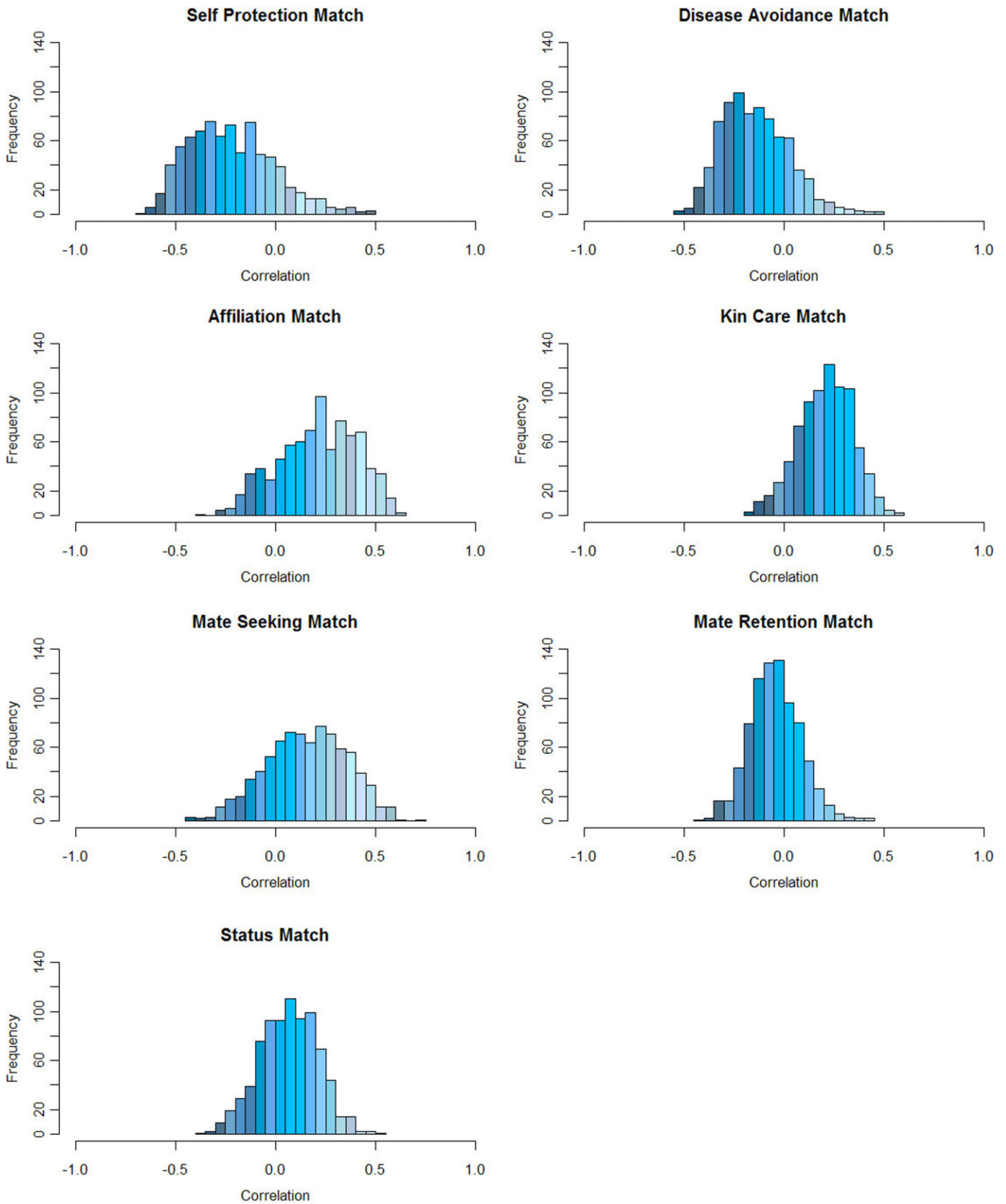
Figure I Histograms of participants' template-match scores, across four visits, for each of seven motive-relevant situation templates.
